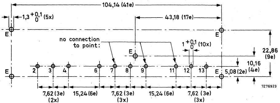
Fig. 3 Piercing diagram viewed from solder side of board; e = 2,54 \text{ mm} (0,1 in). No connection must be made to the points 7, 9 and 11, as otherwise the oscillator radiation would increase.
