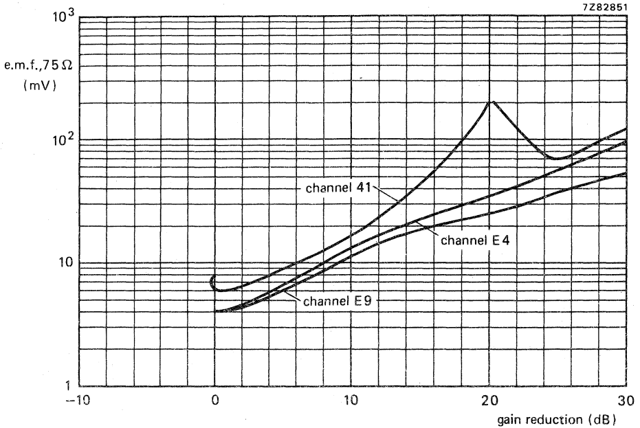
Fig. 11 Cross-modulation, in channel.
