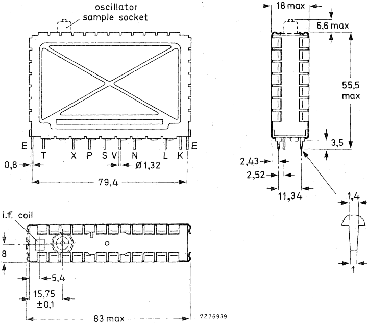
Fig. 2a The oscillator sampling socket, drawn with dotted lines, applies only to tuner V317LO.
