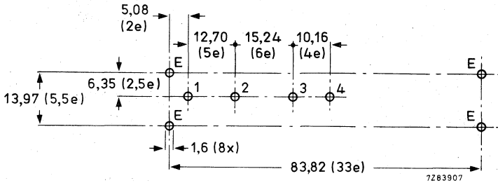
Fig. 2 Piercing diagram viewed from solder side of board; e = 2,54 \text{ mm} ( 0,1 \text{ in} ).
