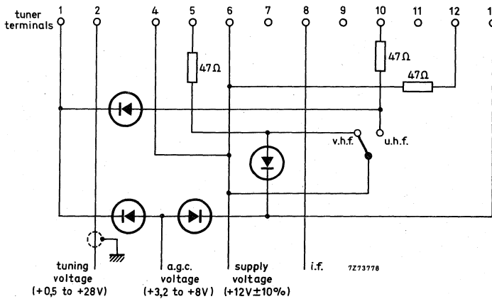
Fig. 13. Connection diagram with one switch.
