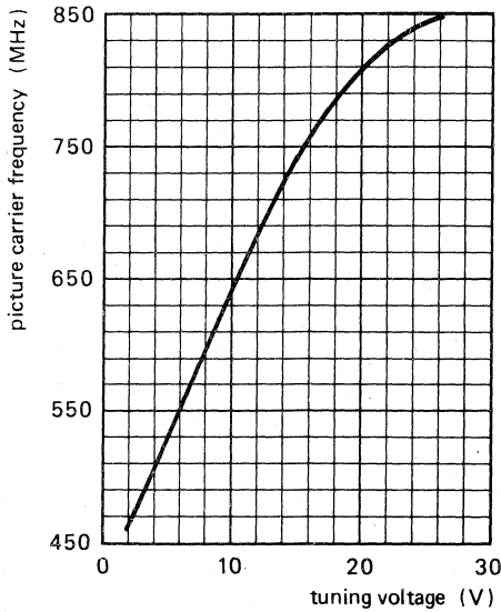
Fig. 9 Typical tuning characteristic, bands IV and V.
