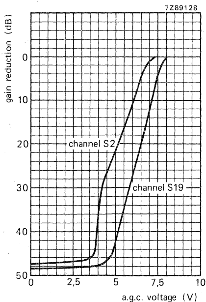
Fig. 5 Typical a.g.c. voltage characteristic, channels S2 and S19.
