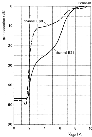
Fig. 6 Typical a.g.c. characteristic, u.h.f.
