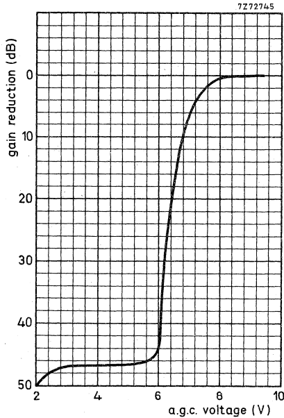
Fig. 4 A.G.C. voltage characteristic, channel E2; typical curve.
