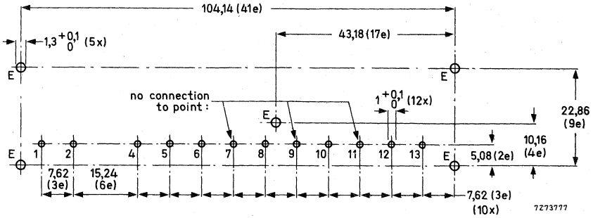
Fig. 3. Piercing diagram viewed from solder side of board; e = 2,54 mm (0,1 in). No connection must be made to the points 7, 9 and 11, otherwise the oscillator radiation may increase.
