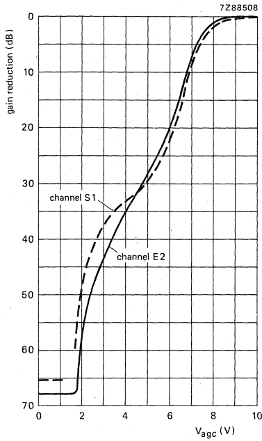
Fig. 4 Typical a.g.c. characteristic, low v.h.f.
