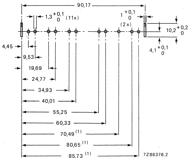
Fig. 3 Piercing diagram viewed from solder side of board. Unless otherwise stated the tolerance is \pm 0,05 mm.
