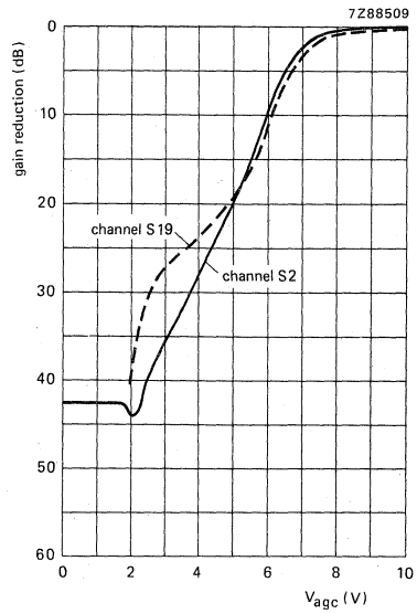
Fig. 5 Typical a.g.c. characteristic, high v.h.f.
