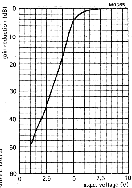
Fig. 4 Typical a.g.c. characteristic, band I.
