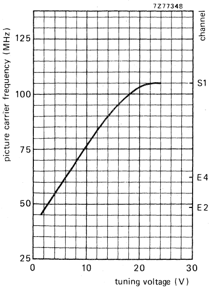
Fig. 8 Typical tuning voltage characteristic, v.h.f. I.
