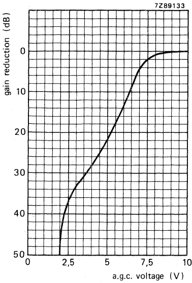
Fig. 6 Typical a.g.c. voltage characteristic, channel E5.
