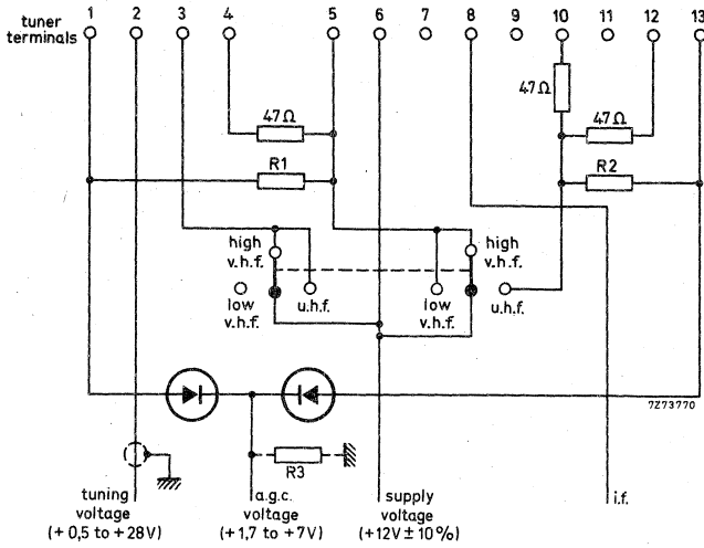
Fig. 16. Connection diagram with two switches. All diodes: BAX13, BA217 or comparable silicon diodes. The values of R 1 , R 2 and R 3 depend on a.g.c. circuit.
