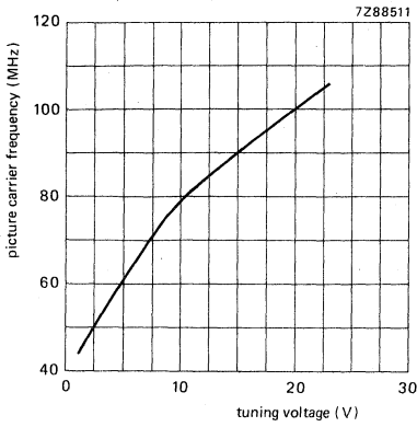
Fig. 7 Typical tuning characteristic, low v.h.f.
