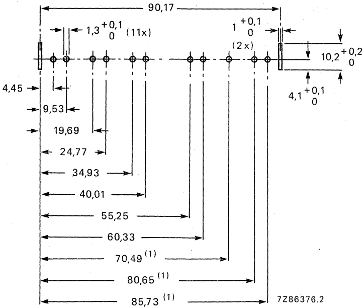
Fig. 3 Piercing diagram viewed from solder side of board. Unless otherwise stated the tolerance is \pm 0,05 \text{ mm} .
