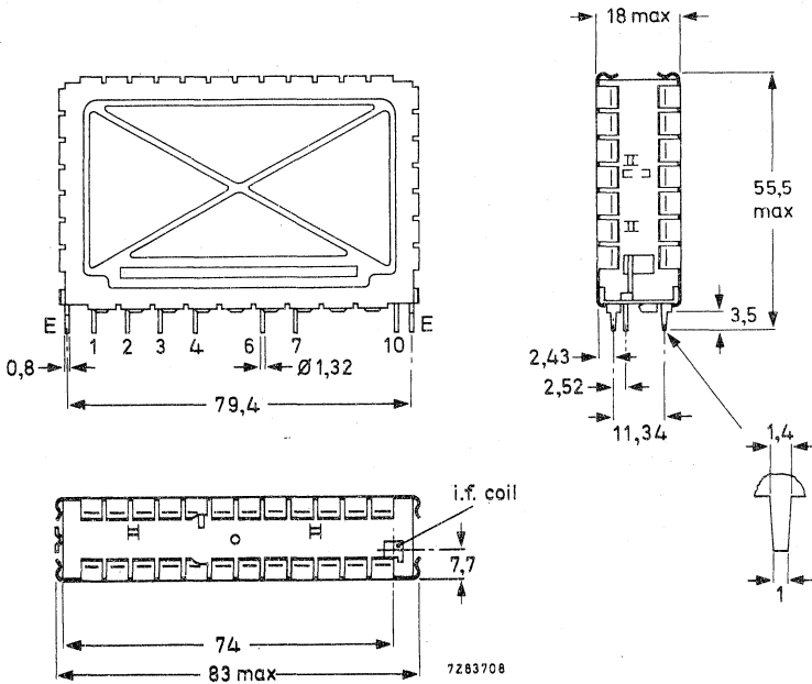
Fig. 2a Terminal 1 = aerial 2 = r.f. supply voltage, + 12 V 3 = a.g.c. voltage, + 5,0 to + 1,0 V 4 = tuning voltage, + 1 to + 28 V 6 = oscillator/i.f. supply voltage, + 12 V 7 = i.f. injection point 10 = i.f. output
