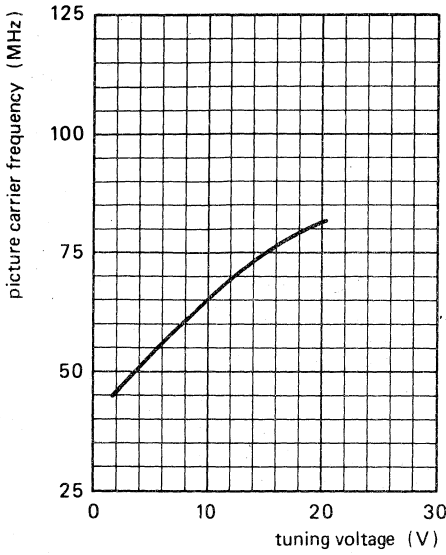
Fig. 7 Typical tuning characteristic, band I.
