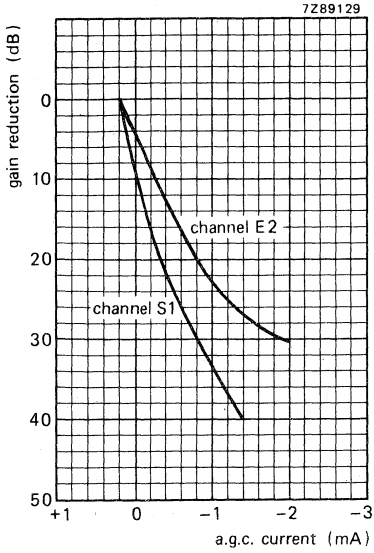
Fig. 6 Typical a.g.c. current characteristic, channels E2 and S1.
