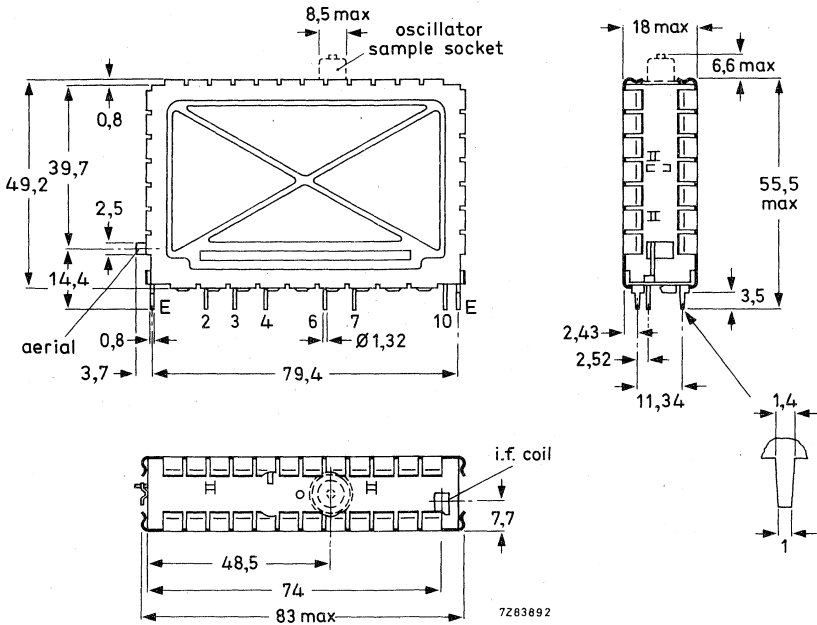
Fig. 2a The oscillator sample socket, drawn with dotted lines, applies only to tuner U341LO.
