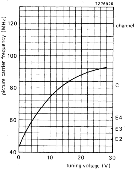
Fig. 8 Typical tuning voltage characteristic, v.h.f. I.
